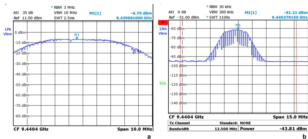
Figure 3 - Peak Power Measurement (a) - Average Power-Channel Power Mode (b)
